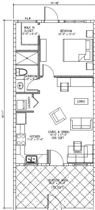
GROUND FLOOR 782 SQFT
